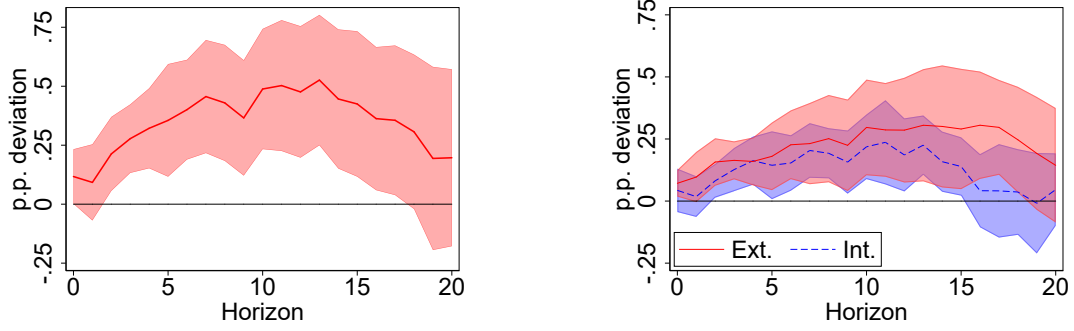
(a) Heterogeneous Effect (Young - Old)
