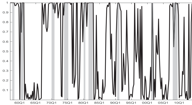
Figure C.1: Regime Probabilities
