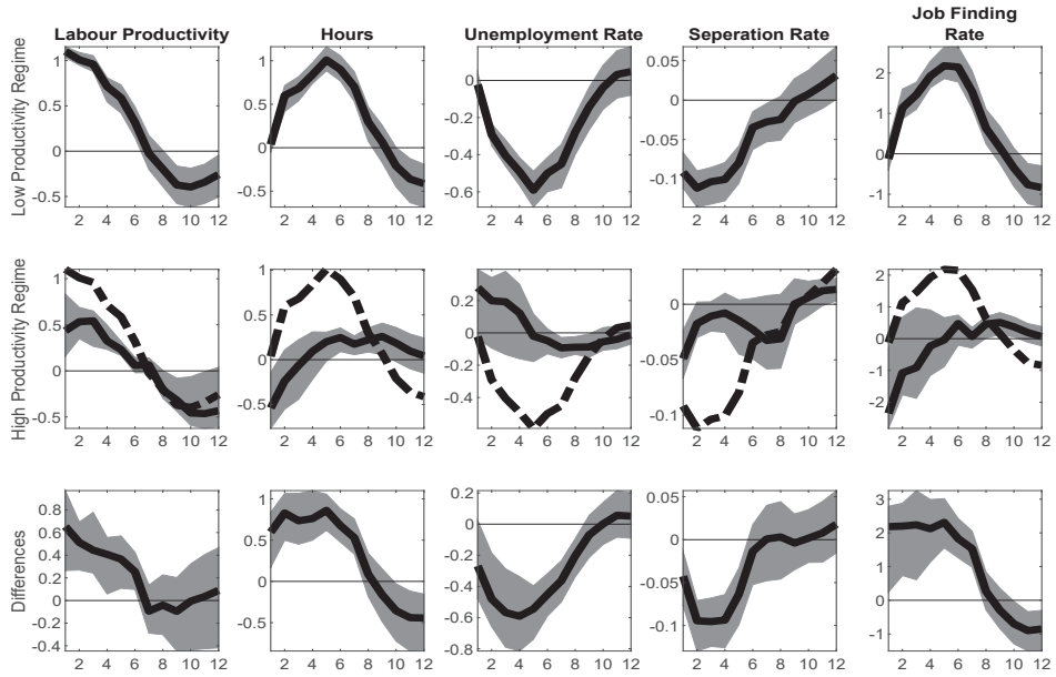
Figure C.2: Impulse Responses
